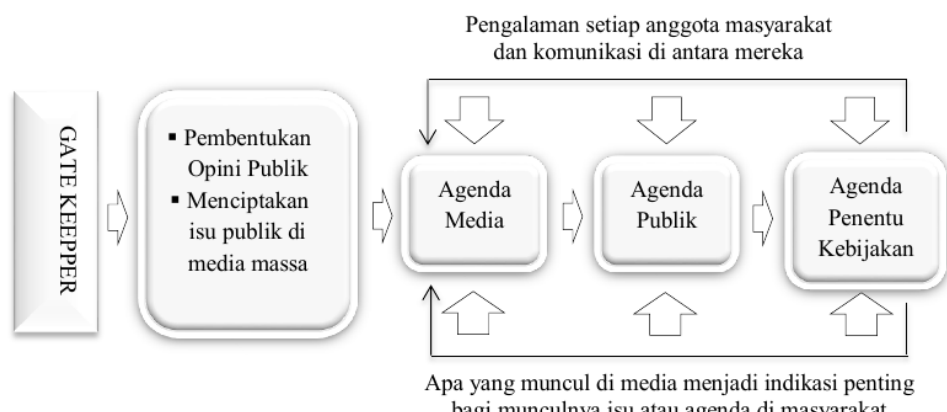
Gambar 2. Proses Agenda-Setting
